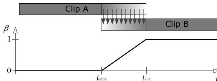
Figure 11.27. A smooth transition, in which the local clocks of both clips keep running during the transition.
