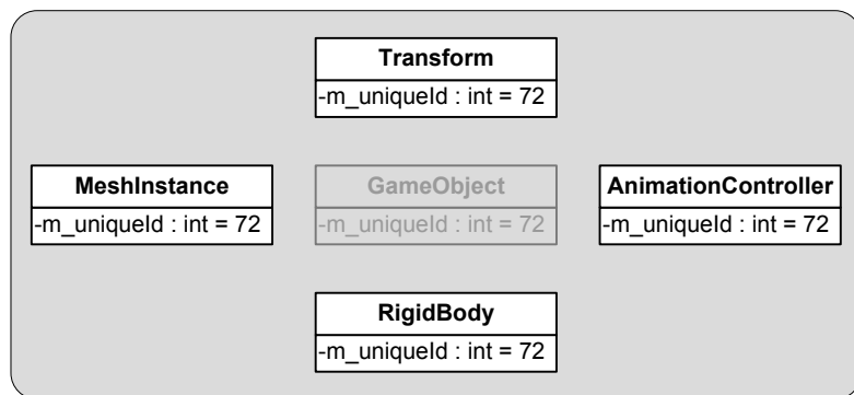
Figure 15.10. In a pure component model, a logical game object is comprised of many components, but the components are linked together only indirectly, by sharing a unique id.
