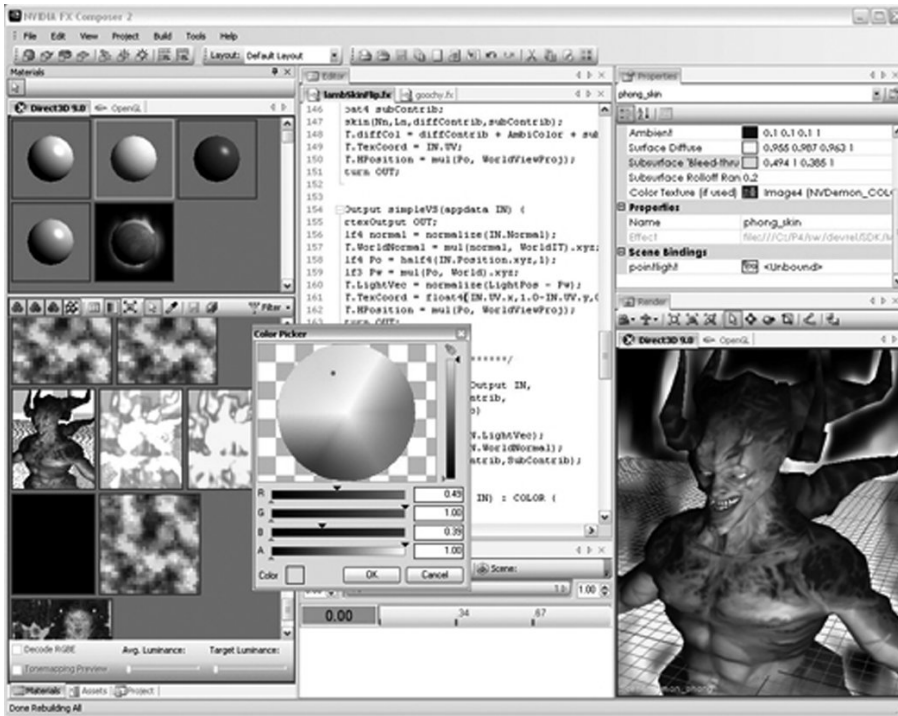
Figure 10.42. Nvidia's Fx Composer allows shader programs to be written, previsualized and debugged easily.
