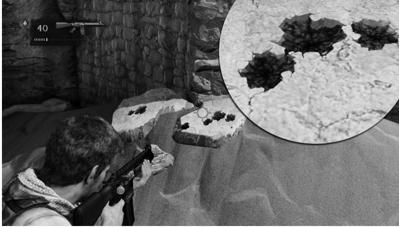
Figure 10.64. Parallax-mapped decals from Uncharted 3: Drake's Deception (© 2011™ SCEA. Created and developed by Naughty Dog, PlayStation 3). (See Color Plate XXIII.)
