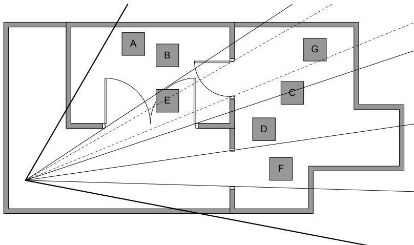
Figure 10.48. Portals are used to define frustum-like volumes, which are used to cull the contents of neighboring regions. In this example, objects A, B and D will be culled because they lie outside one of the portals; the other objects will be visible.
