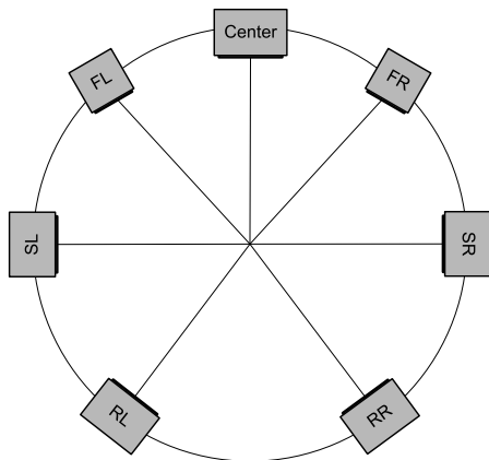
Figure 13.29. Speaker layout for 7.1 pan.
