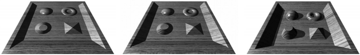
Figure 10.53. Comparison of bump mapping (left), parallax occlusion mapping (center) and displacement mapping (right).
