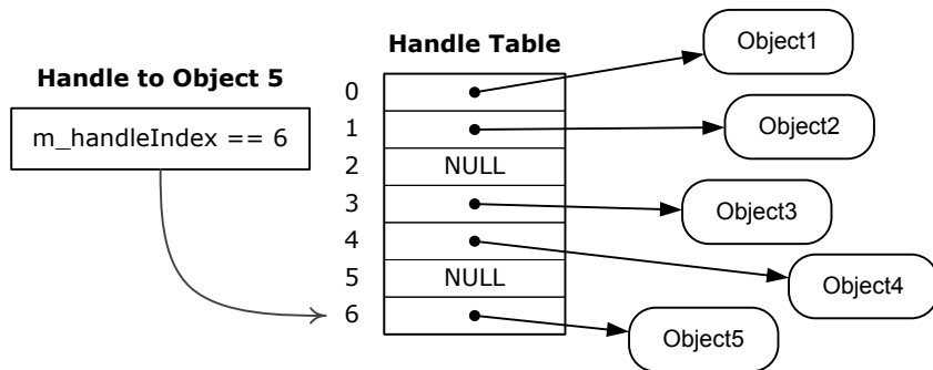
Figure 15.13. A handle table contains raw object pointers. A handle is simply an index into this table.
