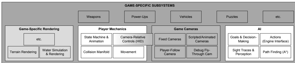
Figure 1.34. Game-specific subsystems.
