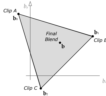
Figure 11.35. Two-dimensional animation blending between three animation clips.
