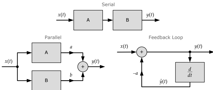
Figure 13.10. Various ways to interconnect systems. In the serial connection, y(t) = B(A(x(t))) . In the parallel connection, y(t) = aA(x(t)) + bB(x(t)) . In the feedback loop, y(t) = x(t) - a\dot{y}(t) .
