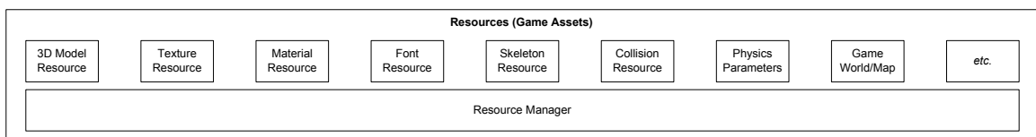
Figure 1.22. Resource manager.
