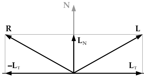
Figure 10.24. Calculation of the reflected lighting vector \mathbf{R} from the original lighting vector \mathbf{L} and the surface normal \mathbf{N} .
