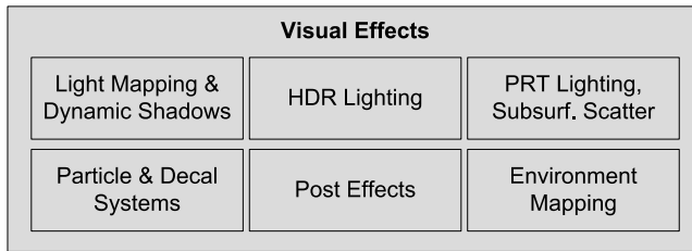
Figure 1.25. Visual effects.
